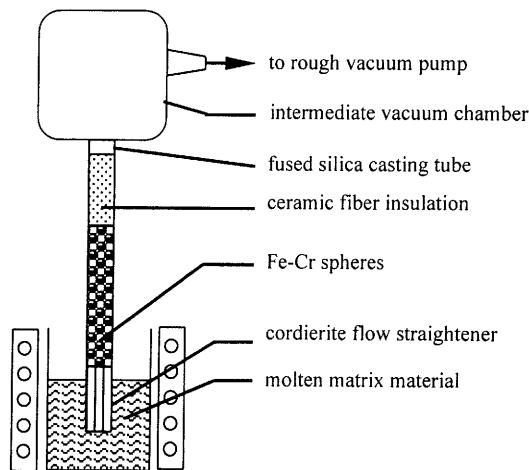
Fig 1: Schematic of aspiration casting apparatus.
