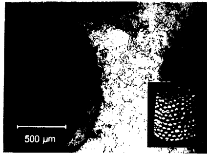
Fig 5: Fe-Cr hollow spheres in AZ31B Mg alloy matrix. Inset: Diffusion bonded preform, ~2 cm diameter.
