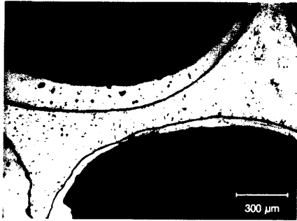
Fig 4: Fe-Cr hollow spheres in a Mg matrix.
